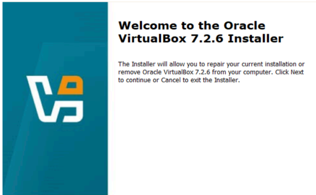
Fig 1.1: Virtualbox Installation
