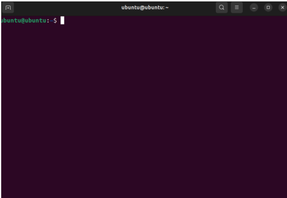
Fig 1.3:Ubuntu terminal
